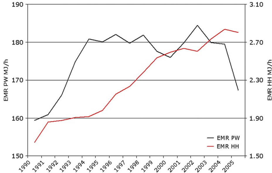
Fig. 2. Exosomatic metabolic rate (energy consumption per hour) of sectors generating added value ( EMR_{PW} ) and sectors consuming added value, households ( EMR_{HH} ), in MJ/h.
