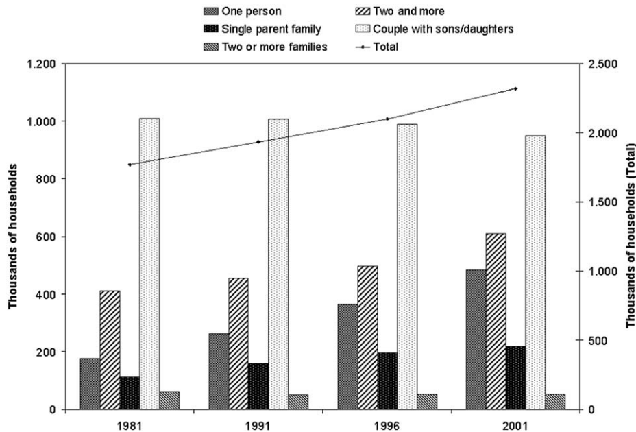
Fig. 3. Household typologies.
